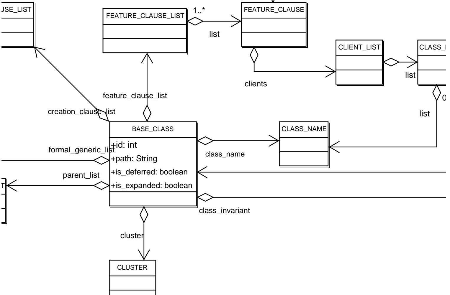
class diagram 1
