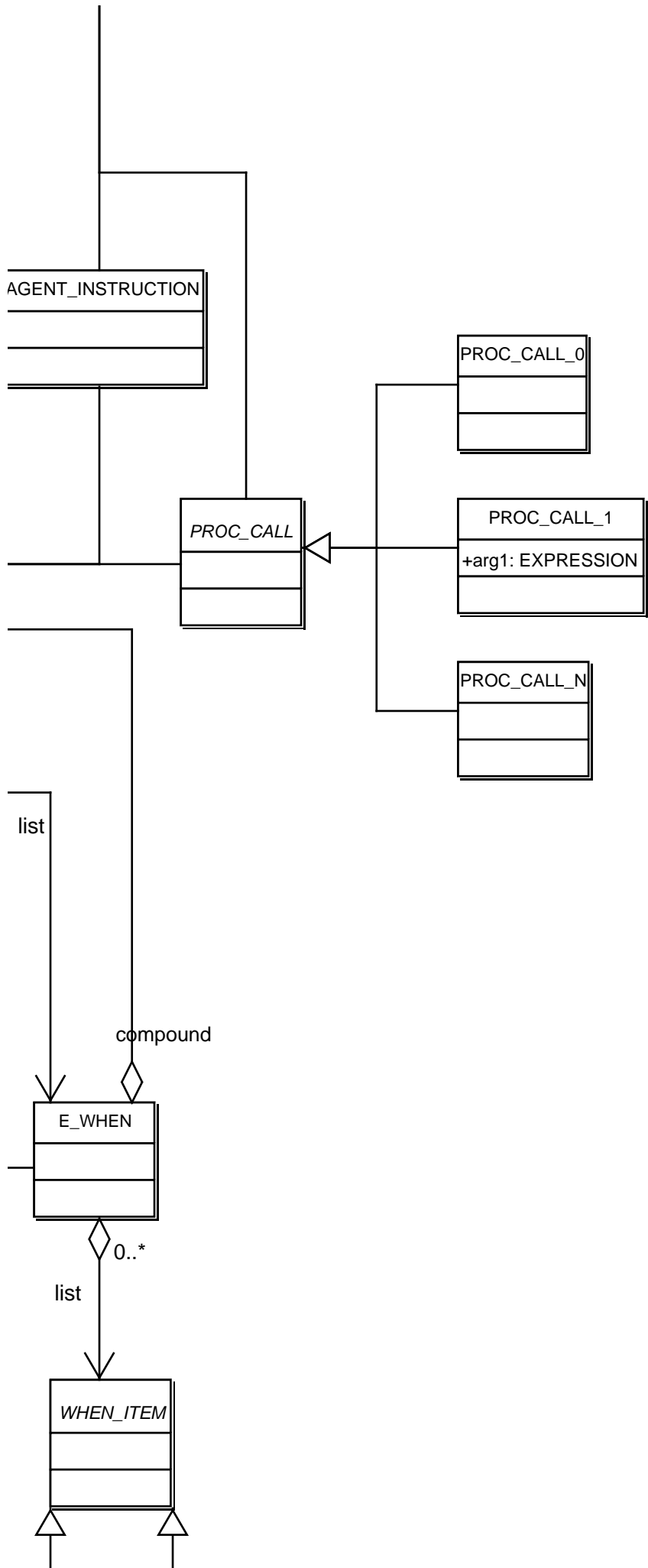
class diagram 1
