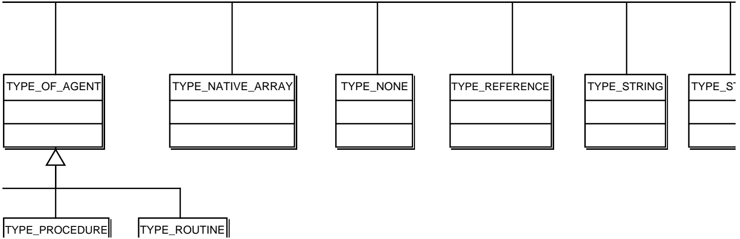
class diagram 1
